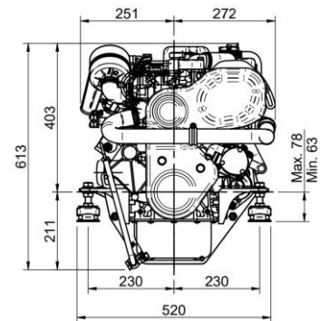
Motor MINI-33 v6 Inv.TMC-40P 2,00:1
